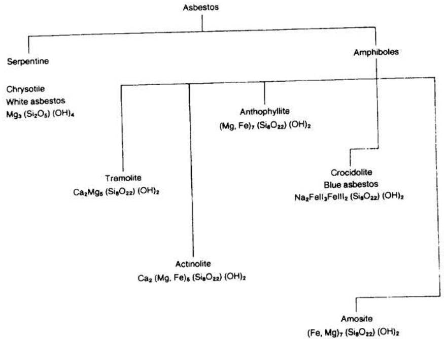
FIGURE 1.—Principal varieties of asbestos
